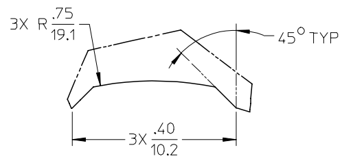
DETAIL1 SCALE 5:1
